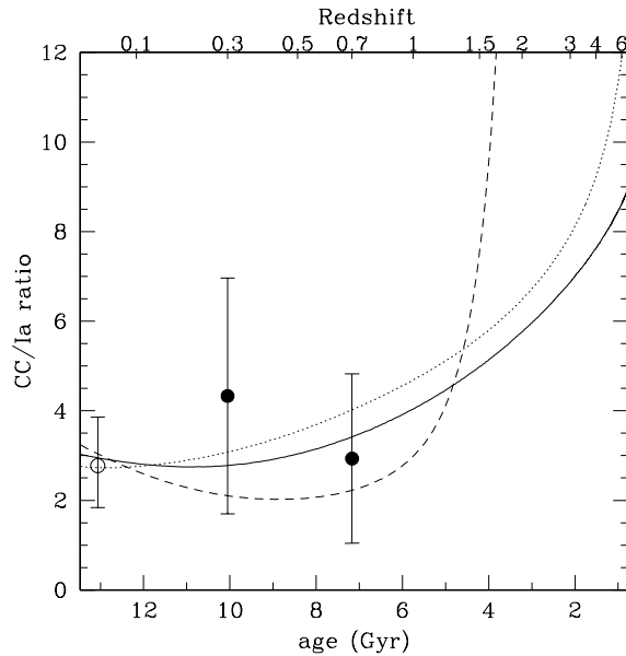
FIGURE 2. Ratio of the rates of the CC to Ia SNe as a function of the redshift. The white and black dots are observed values (Mannucci et al. 2005, Dahlen et al. 2004). The lines show the predictions of the gaussian “single-population” model (i.e. a model in which the DTD is a narrow gaussian centered at 3-4 Gyr; dashed line), Yungelson and Livio (2000) DD Chandrasekar mass model (dotted line), and the “two-populations” shown in Figure 1 (solid line). The predictions use a Salpeter IMF and mass ranges of 3-8 M_{\odot} (SNIa) and 8-40 M_{\odot} (CC SNe), and are scaled to match the observed values.
